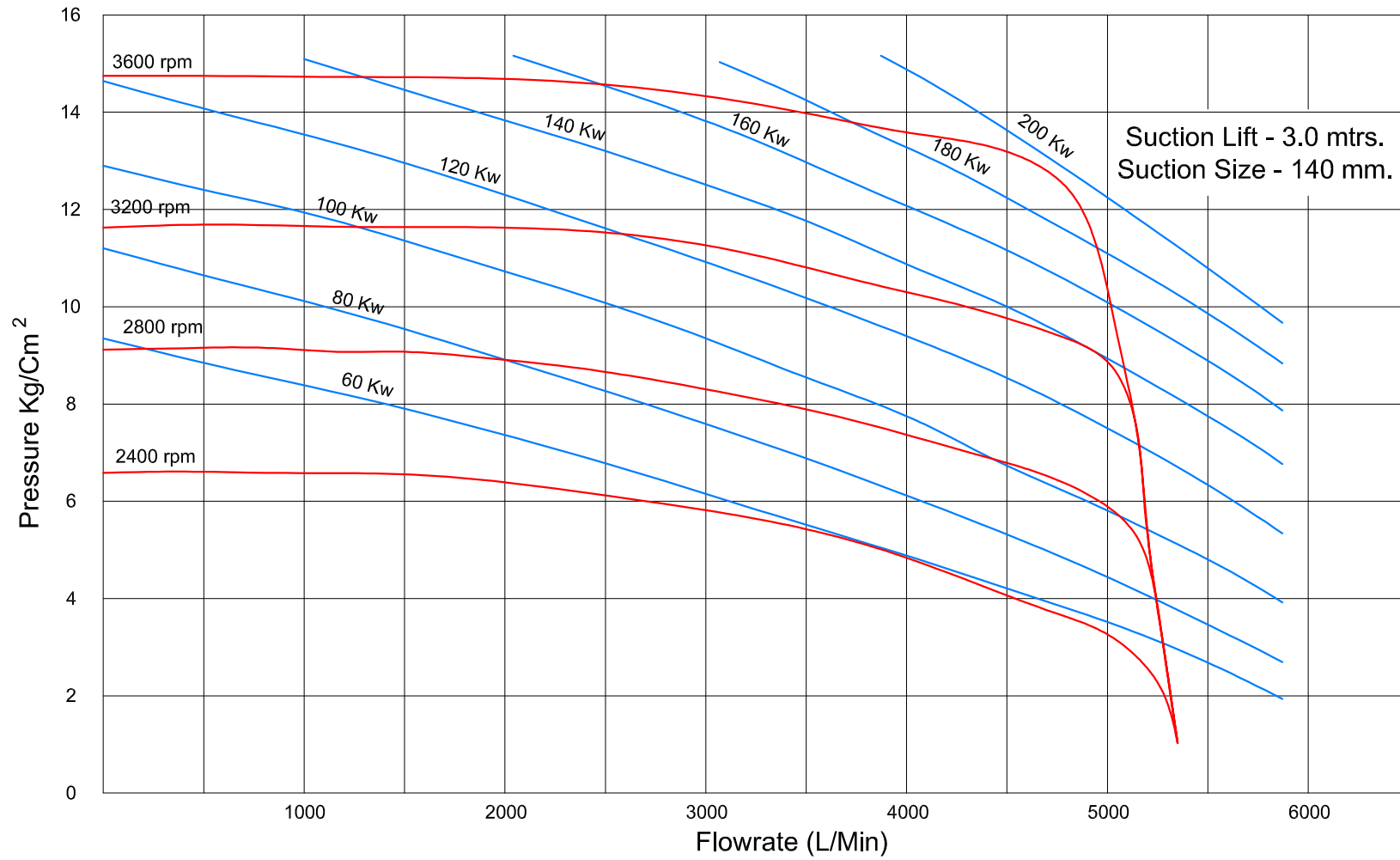
Typical Low Pressure Performance of MFV MP 1040
