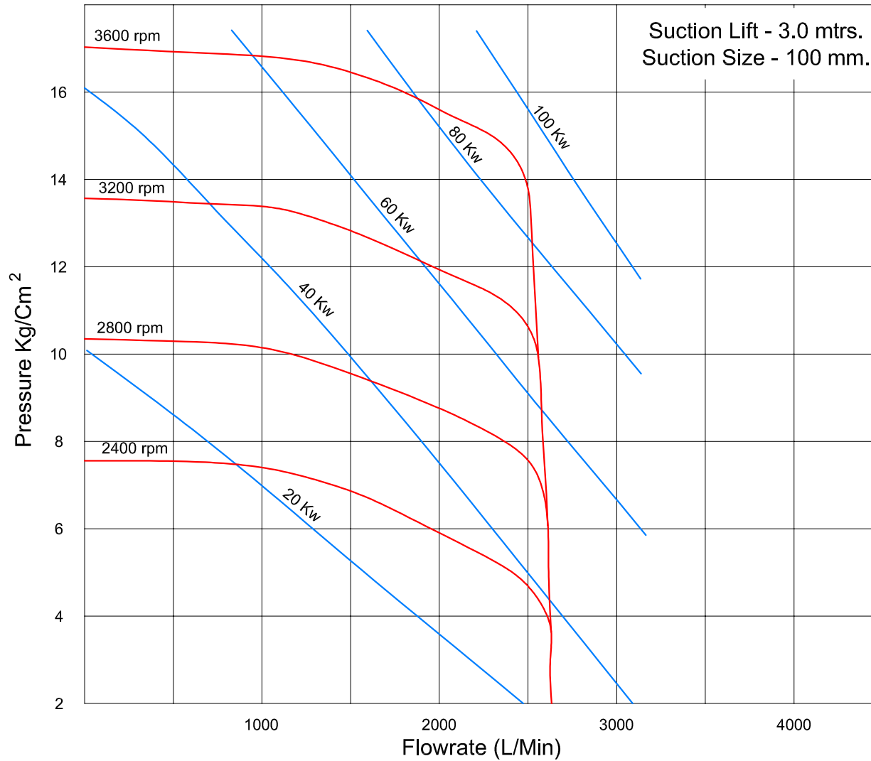
Typical Performance of MFV LP 1020
